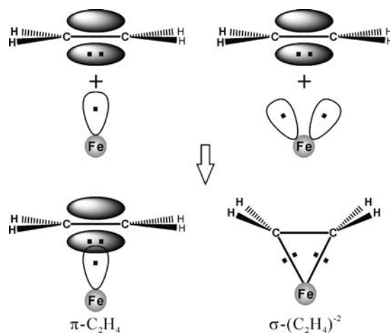
FIGURE 6. Cartoon representation of alternate schemes for binding C 2 H 4 to a cofactor metal ion: (left) dative π bonding; (right) oxidative addition to form Fe–C σ bonds.
